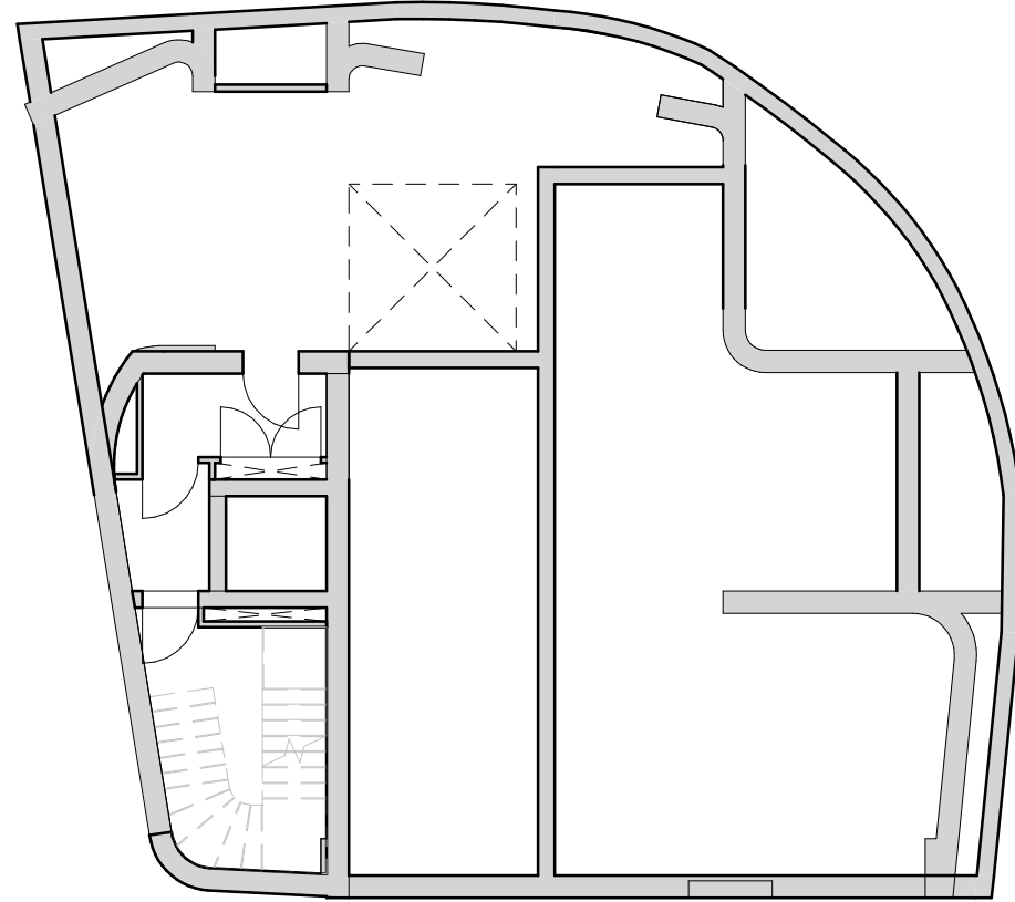
BASEMENT -3
