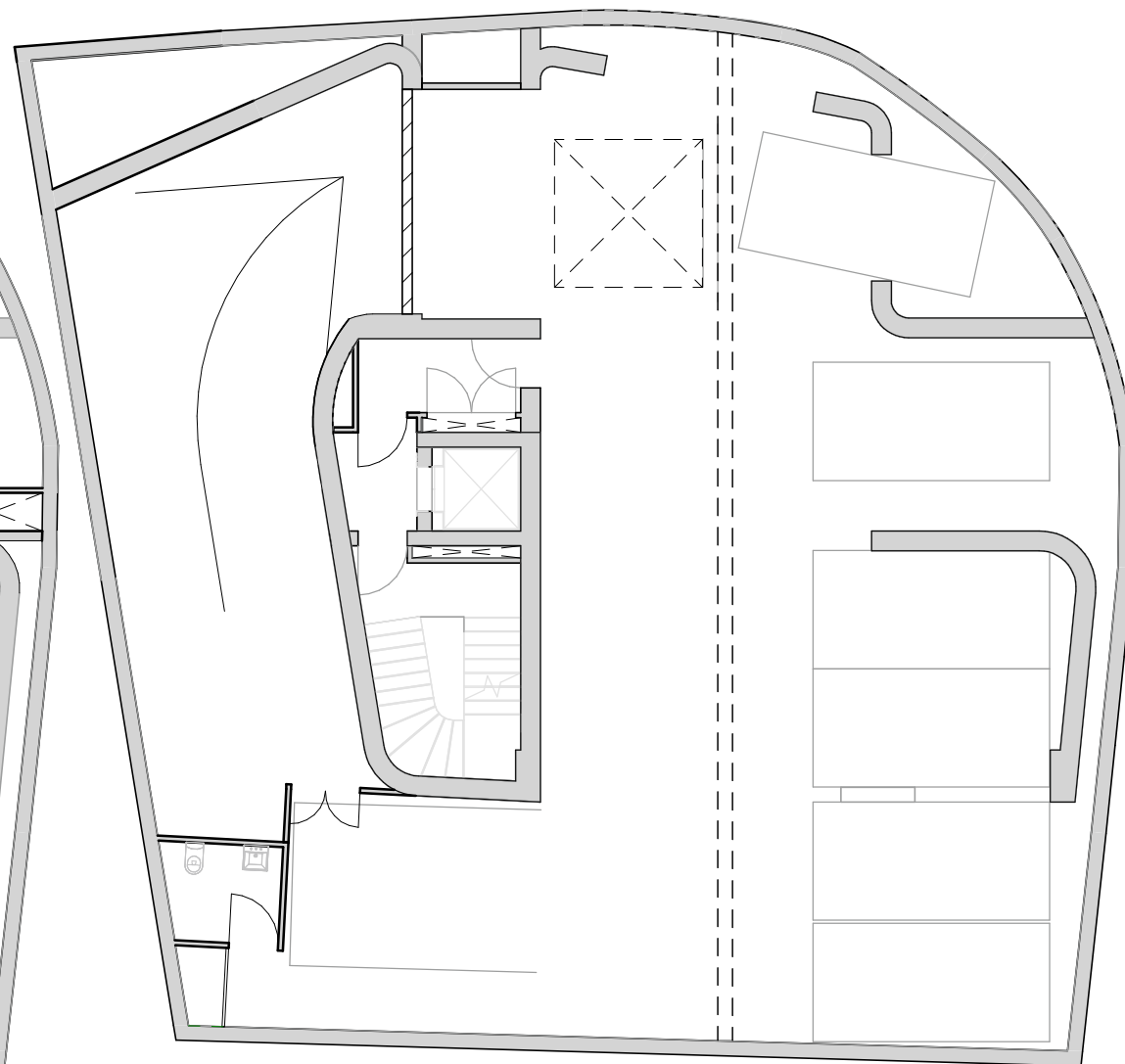
BASEMENT -2
